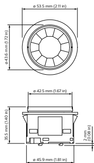
LRM1657/05 ActiLume 1-10V Ind Mov Sensor
