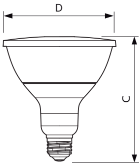
MAS LEDspot D 13-100W E27 927 PAR38 25D
