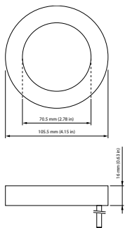
LCU7591 Amplight Leak Coil
