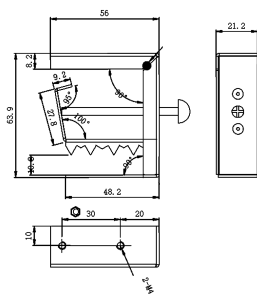
Mechanical accessory
