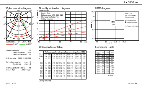
IFGU_4MX900 G3 581 1xLED50S/840 PSD MB-General uniform lighting
