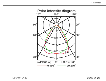
IFPC1_4MX900 G3 581 1xLED50S/840 PSD MB.EPS
