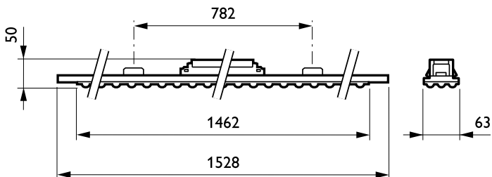
Maxos LED electr. units 4MX850-883
